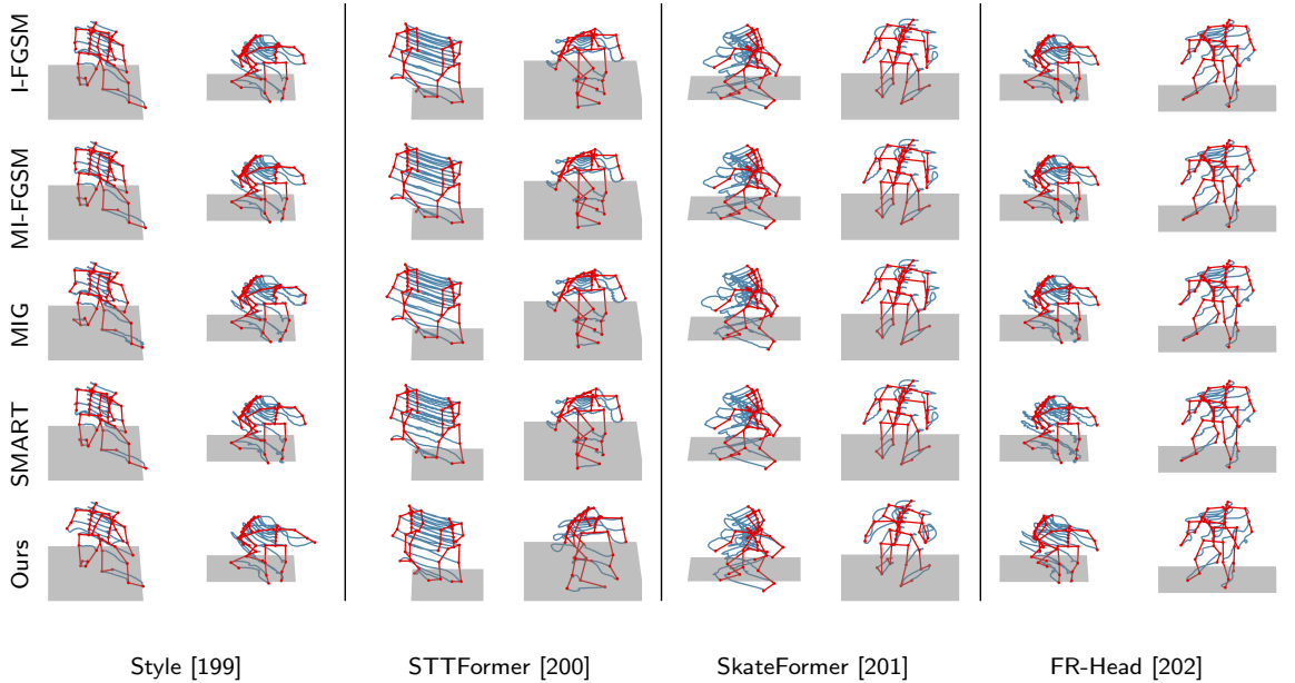
Figure 5.5: Visual comparison among the adversarial motions generated by different attack methods against victim models. We visualize the starting and the ending poses in red, the trajectories of all joints in blue, and the ground floor in grey. Our adversarial motions exhibit the most smooth and stable trajectories.
