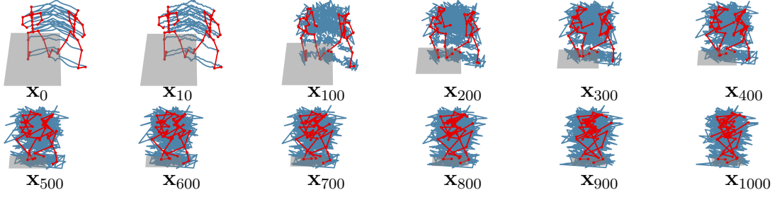
Figure 5.1: The visualization of diffusion latents at different timesteps. As shown, the earlier timesteps maintain more low-level details, the later timesteps focus on high-level structures until latents become pure noise.
