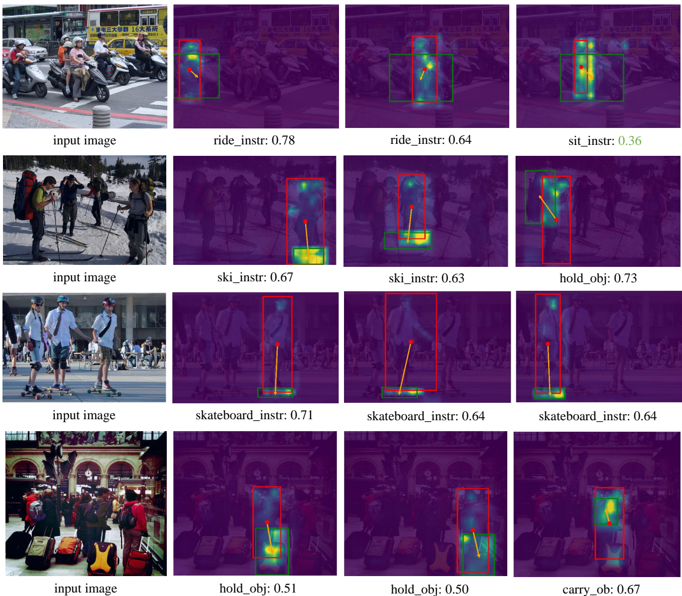
Fig. 1. Qualitative results of GeoHOI. The black prediction scores represent true positive interactions and the green ones indicate true negative interactions.
