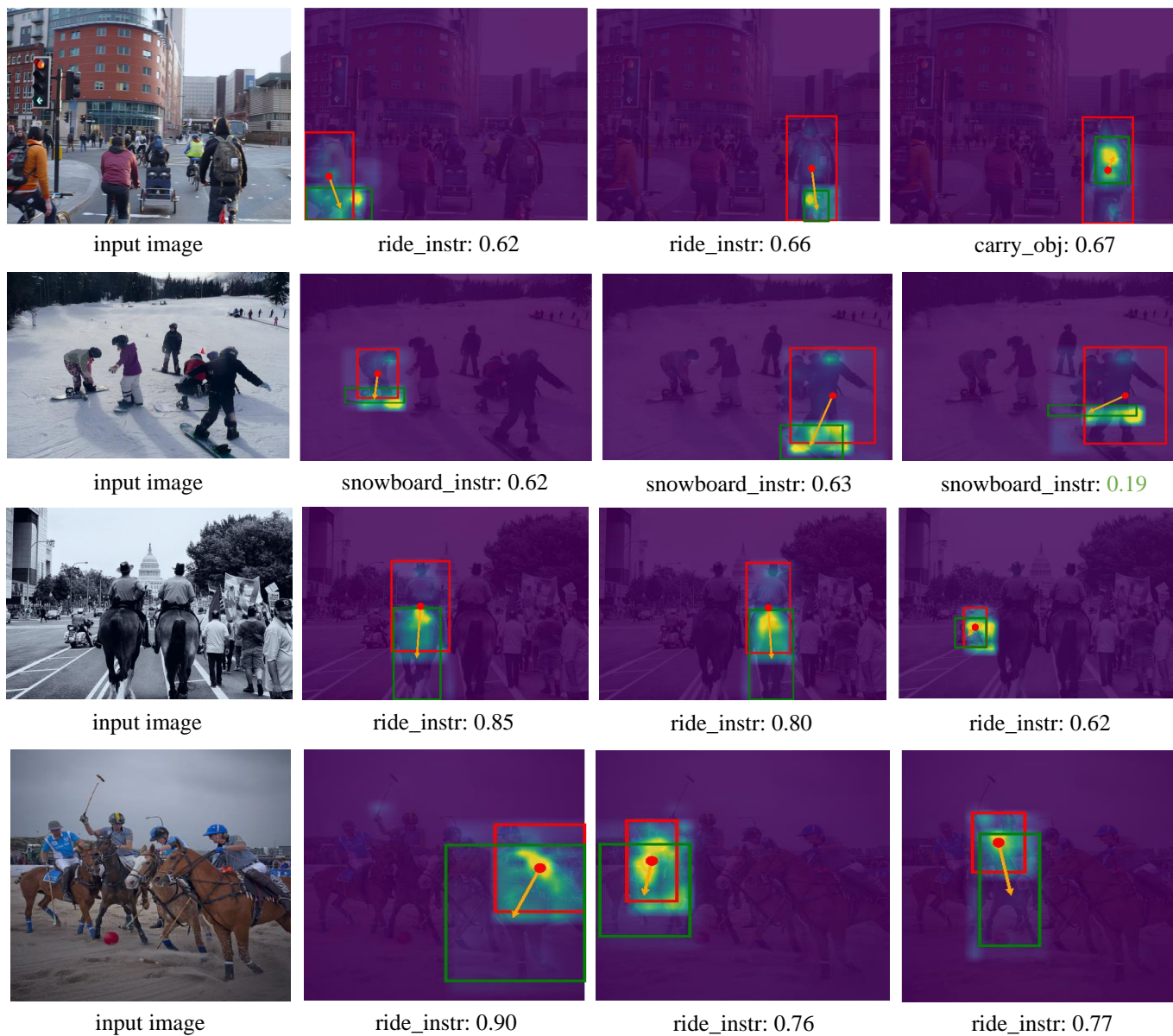
Fig. 2. Qualitative results of GeoHOI. The black prediction scores represent true positive interactions and the green ones indicate true negative interactions.
